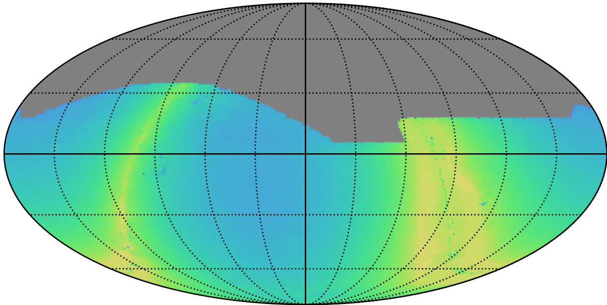
ddf_acor_sf20_lsf0_lsr0_v3.4_10yrs r: N stars to Precision 0.20
