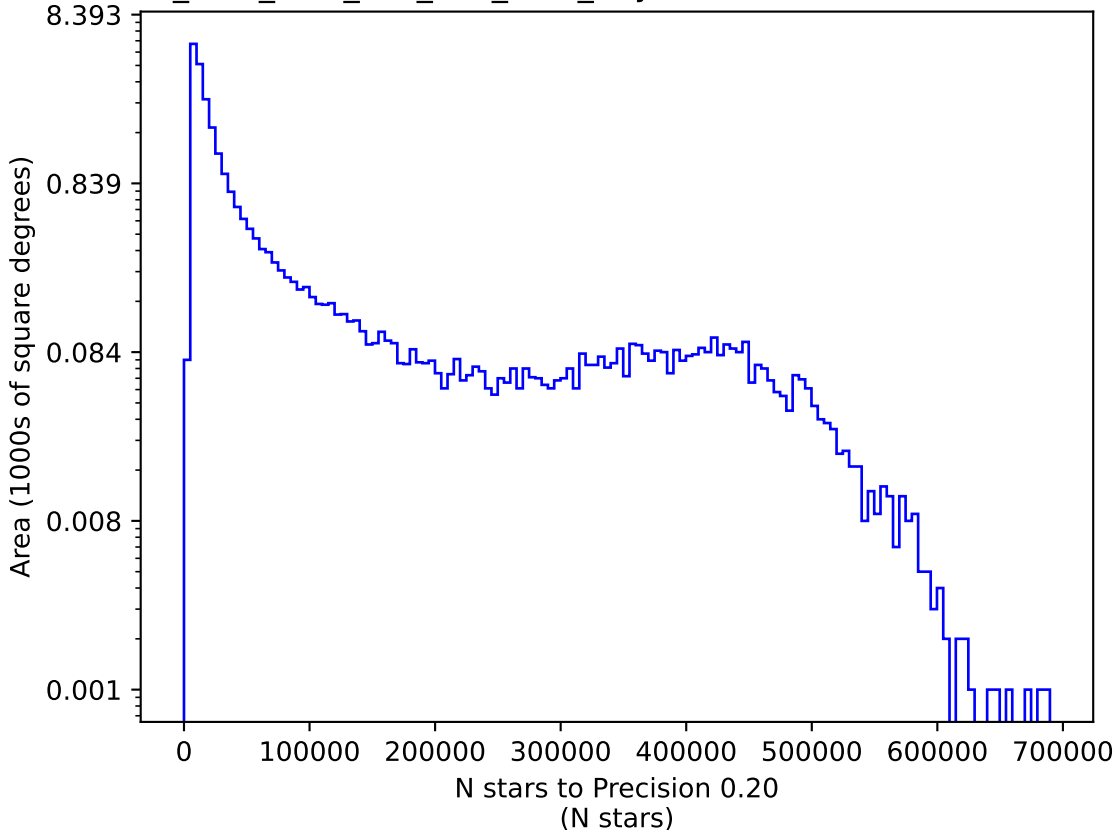
ddf_acor_sf20_ls0_lsr0_v3.4_10yrs i: N stars to Precision 0.20
