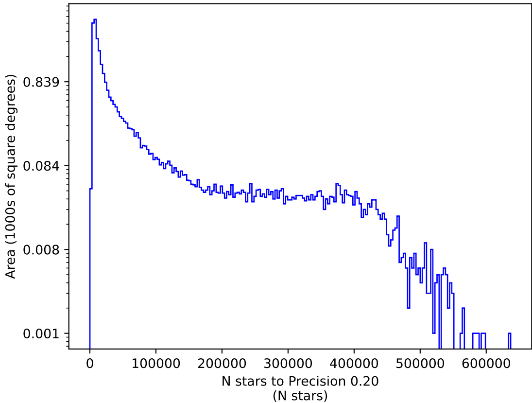
ddf_acor_sf20_lsf0_lsr0_v3.4_10yrs g: N stars to Precision 0.20
