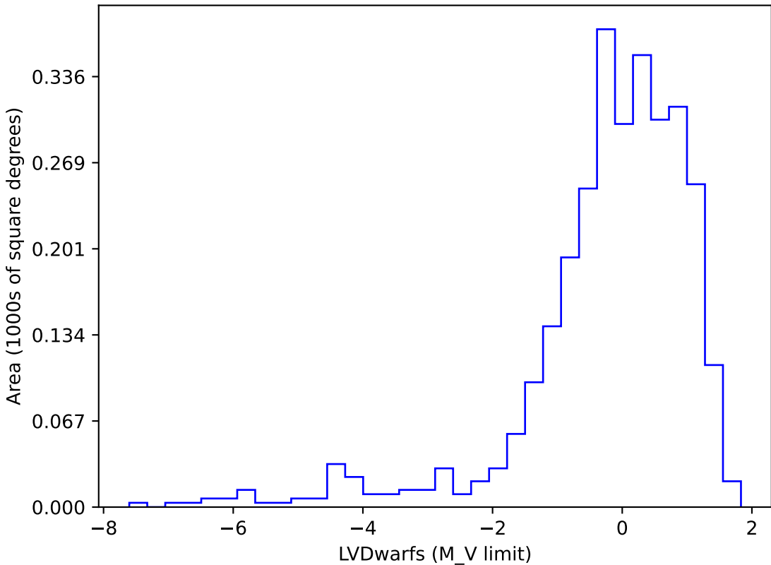
ddf_acor_sf20_lsf0_lsr0_v3.4_10yrs gi SCP: LVDwarfs
