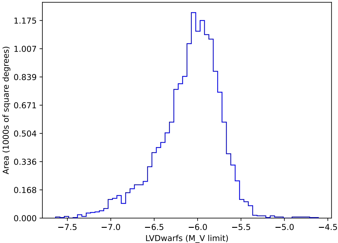
ddf_acor_sf20_lsf0_lsr0_v3.4_10yrs gi: LVDwarfs
