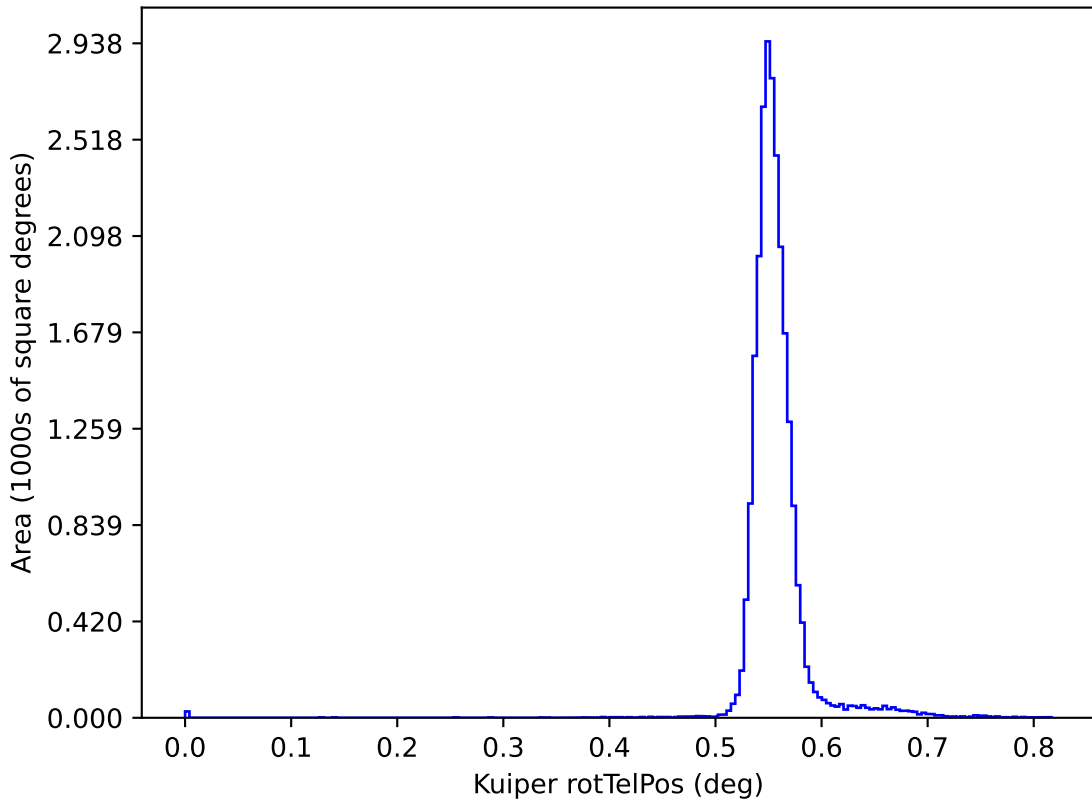
ddf_acor_sf20_lsf0_lsr0_v3.4_10yrs y: Kuiper rotTelPos
