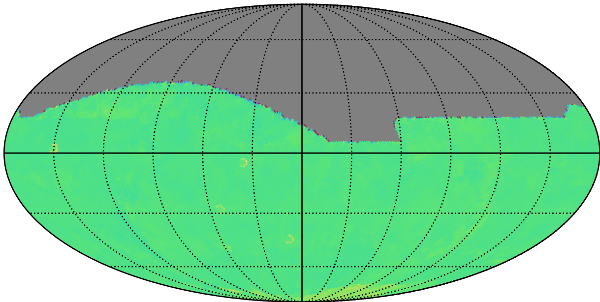
ddf_acor_sf20_lsf0_lsr0_v3.4_10yrs r: Kuiper rotTelPos
