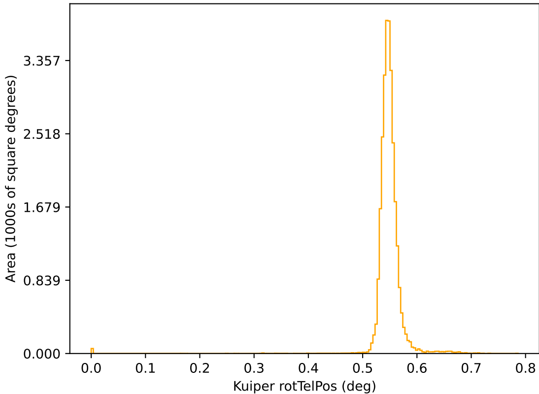
ddf_acor_sf20_ls0_lsr0_v3.4_10yrs r: Kuiper rotTelPos
