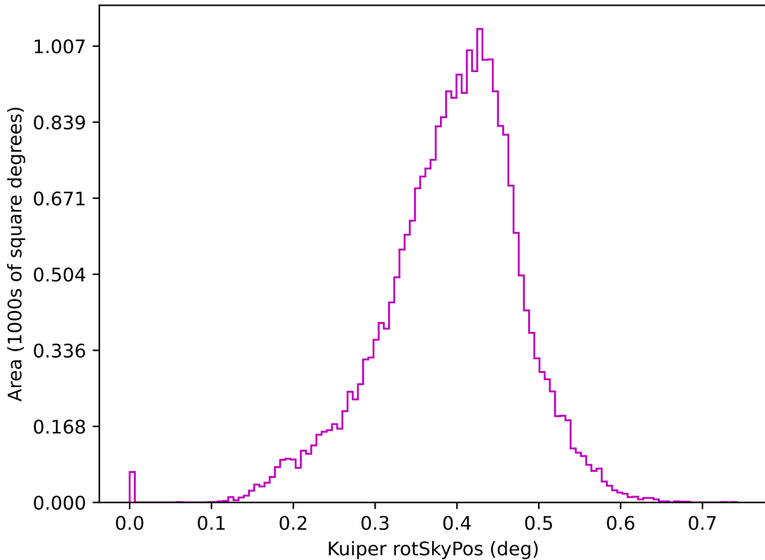
ddf_acor_sf20_lsf0_lsr0_v3.4_10yrs z: Kuiper rotSkyPos
