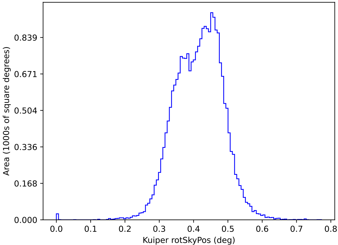
ddf_acor_sf20_lsf0_lsr0_v3.4_10yrs y: Kuiper rotSkyPos
