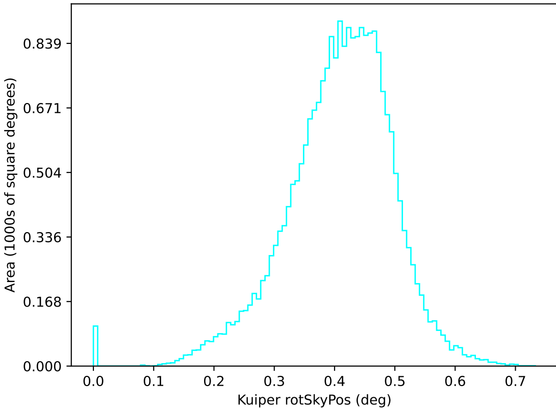
ddf_acor_sf20_lsf0_lsr0_v3.4_10yrs u: Kuiper rotSkyPos
