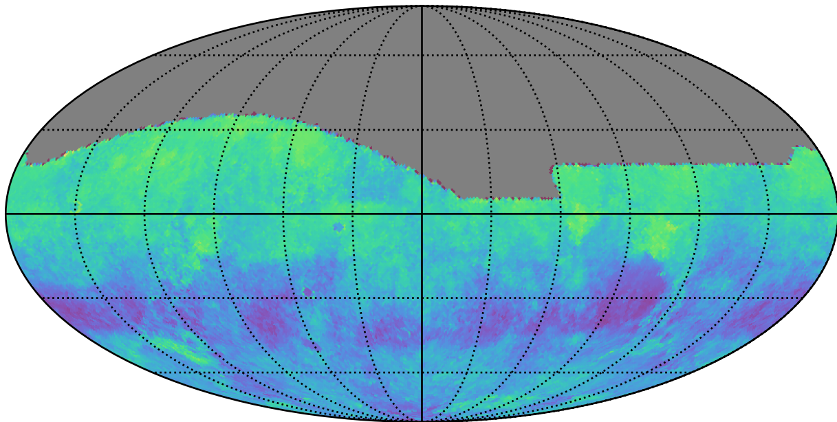
ddf_acor_sf20_lsf0_lsr0_v3.4_10yrs g: Kuiper rotSkyPos
