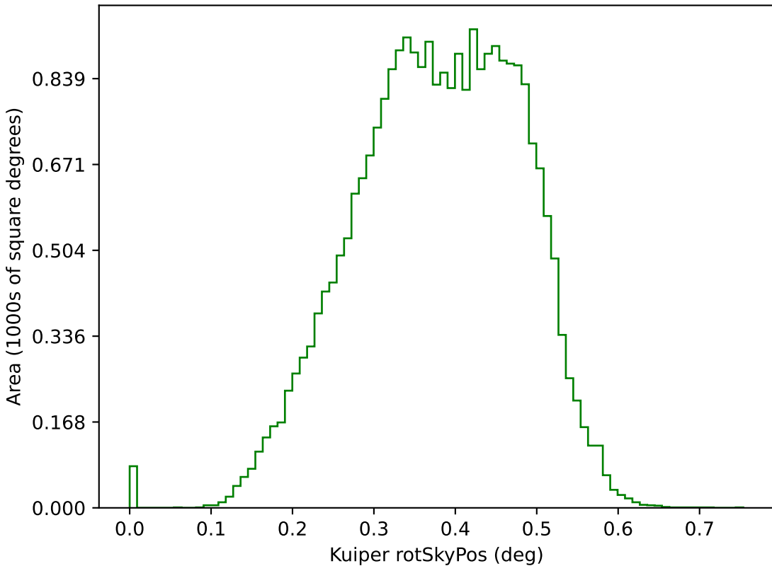
ddf_acor_sf20_lsf0_lsr0_v3.4_10yrs g: Kuiper rotSkyPos
