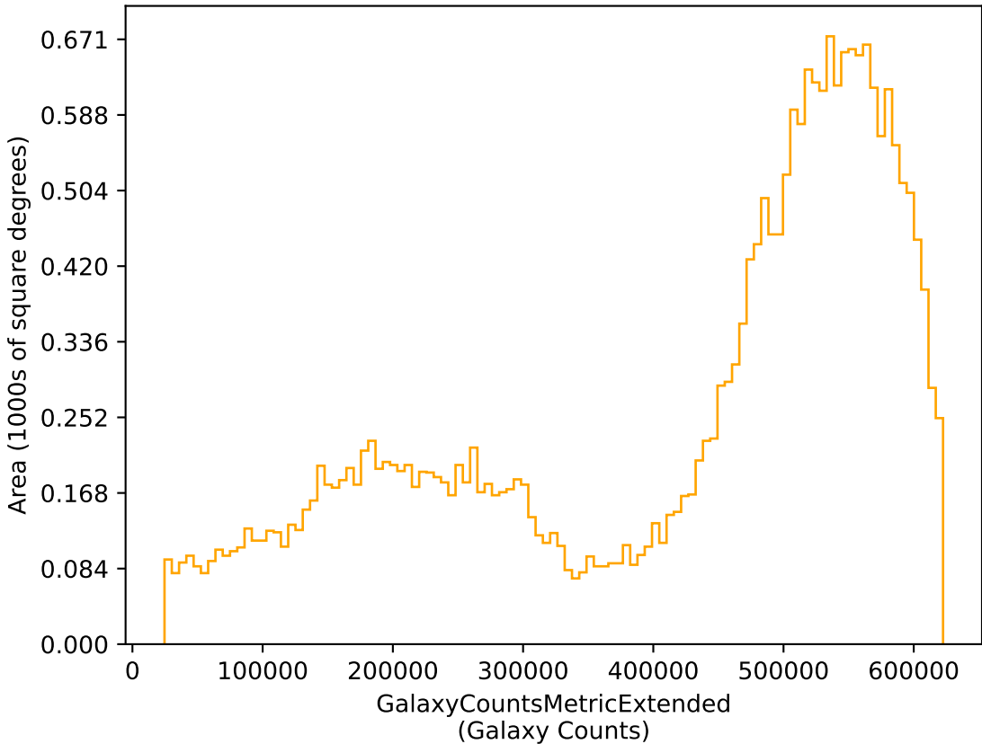
ddf_acor_sf20_lsf0_lsr0_v3.4_10yrs r: GalaxyCountsMetricExtended
