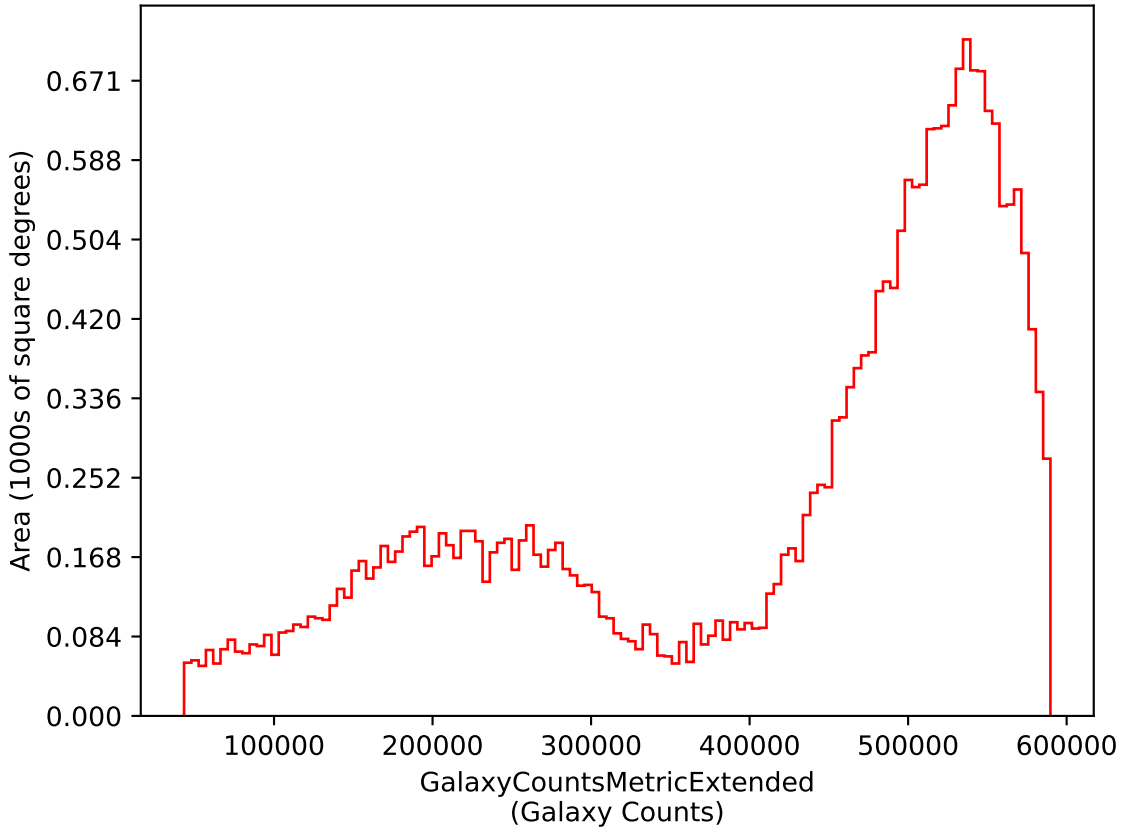
ddf_acor_sf20_lsf0_lsr0_v3.4_10yrs i: GalaxyCountsMetricExtended
