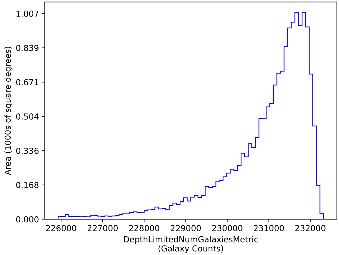
ddf_acor_sf20_lsf0_lsr0_v3.4_10yrs i band galaxies non-DD: DepthLimitedNumGalaxiesMetric
