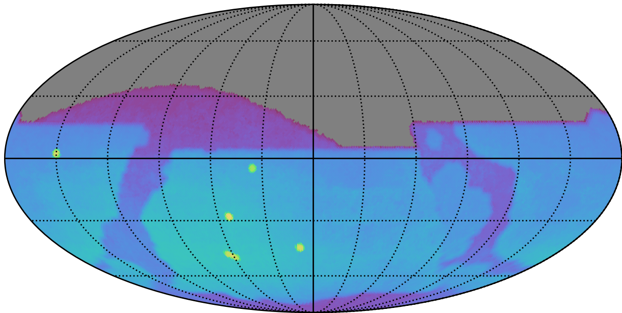
ddf_acor_sf20_lsf0_lsr0_v3.4_10yrs : Brown Dwarf, L7
