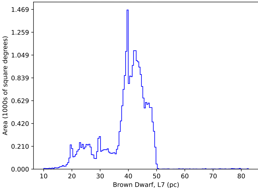
ddf_acor_sf20_ls0_lsr0_v3.4_10yrs : Brown Dwarf, L7
