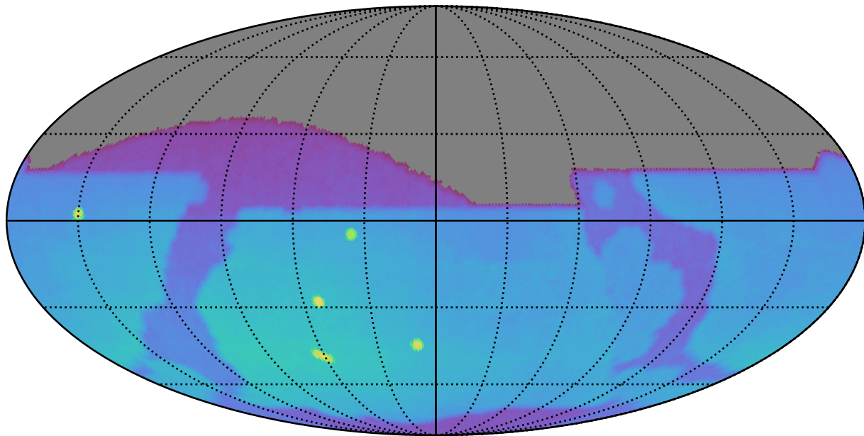
ddf_acor_sf20_lsf0_lsr0_v3.4_10yrs : Brown Dwarf, L4
