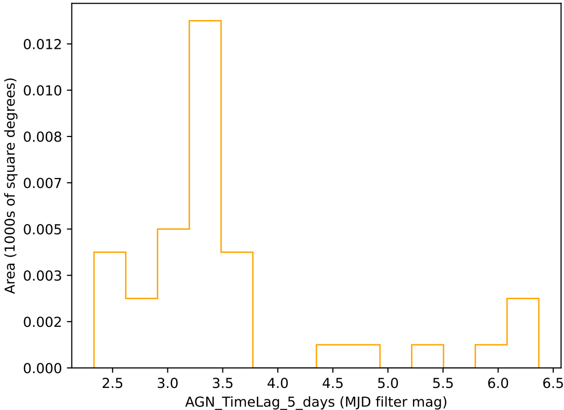
ddf_acor_sf20_lsf0_lsr0_v3.4_10yrs r band: AGN_TimeLag_5_days
