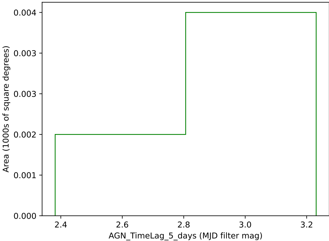
ddf_acor_sf20_lsf0_lsr0_v3.4_10yrs g band: AGN_TimeLag_5_days
