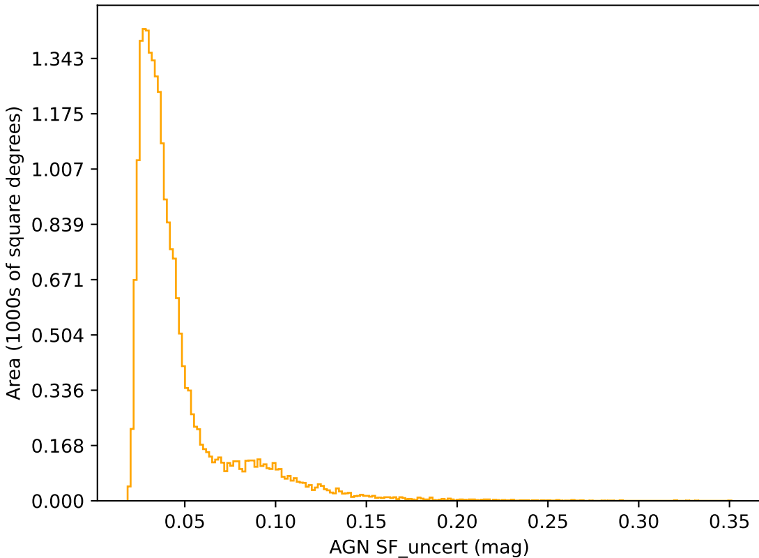
ddf_acor_sf20_lsf0_lsr0_v3.4_10yrs r band: AGN SF_uncert
