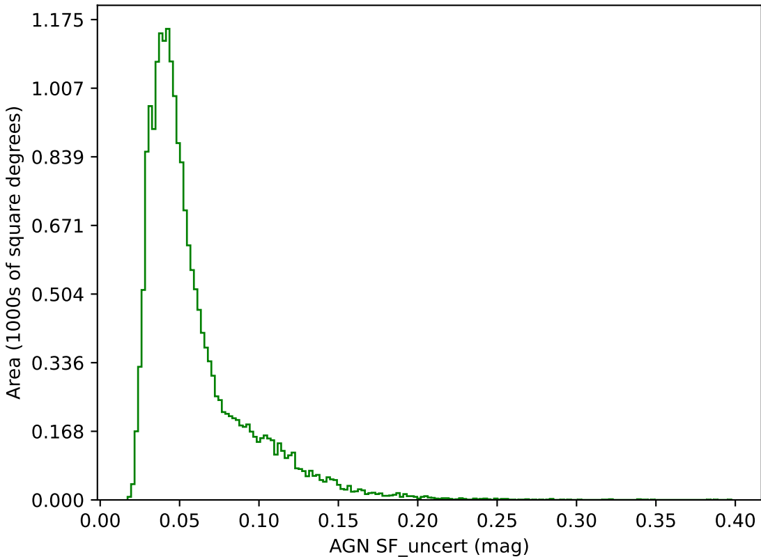
ddf_acor_sf20_lsf0_lsr0_v3.4_10yrs g band: AGN SF_uncert
