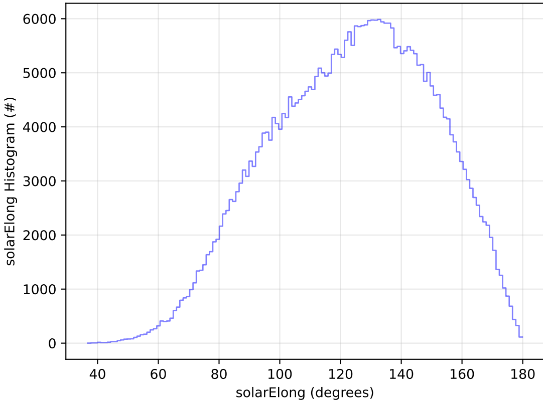
ddf_acor_sf20_lsf0_lsr0_v3.4_10yrs WFD y band: solarElong Histogram
