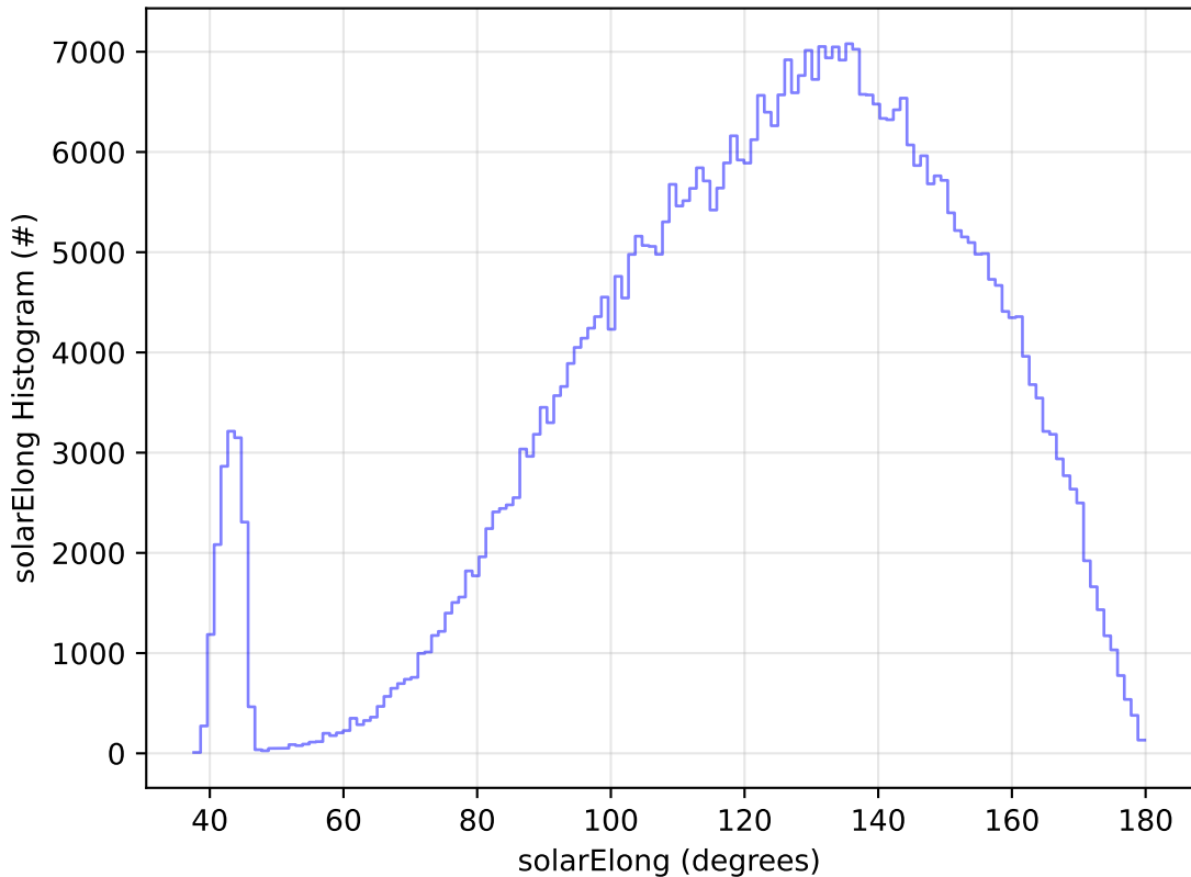
ddf_acor_sf20_lsf0_lsr0_v3.4_10yrs WFD r band: solarElong Histogram
