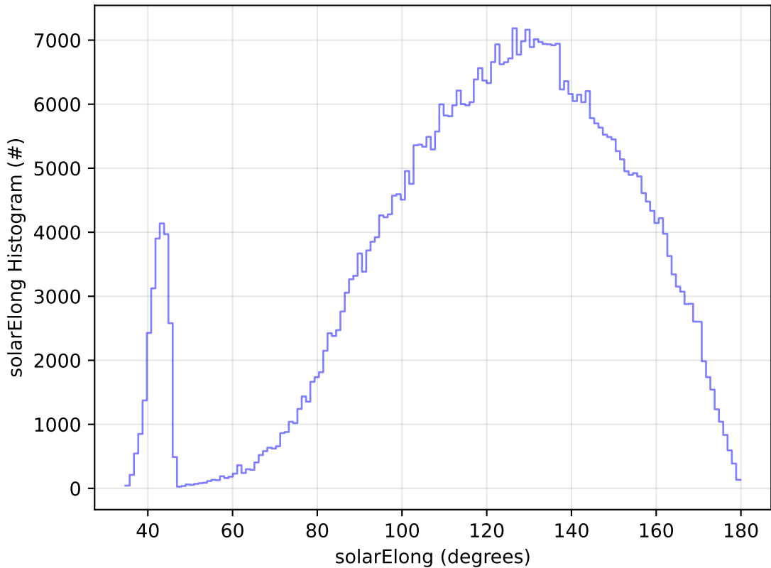
ddf_acor_sf20_lsf0_lsr0_v3.4_10yrs WFD i band: solarElong Histogram
