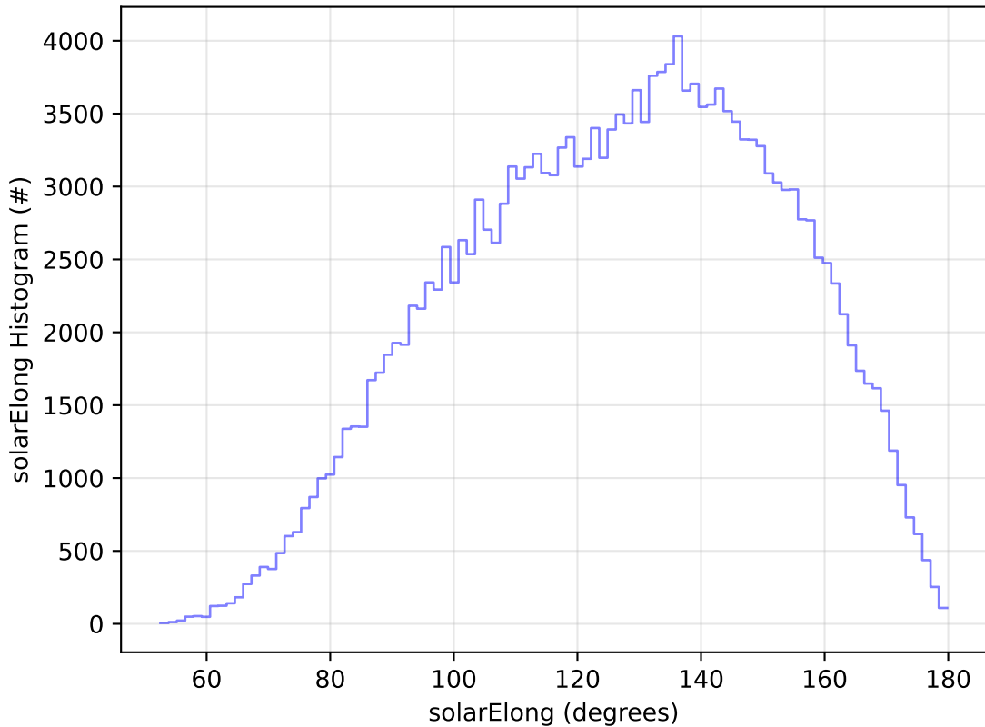
ddf_acor_sf20_lsf0_lsr0_v3.4_10yrs WFD g band: solarElong Histogram
