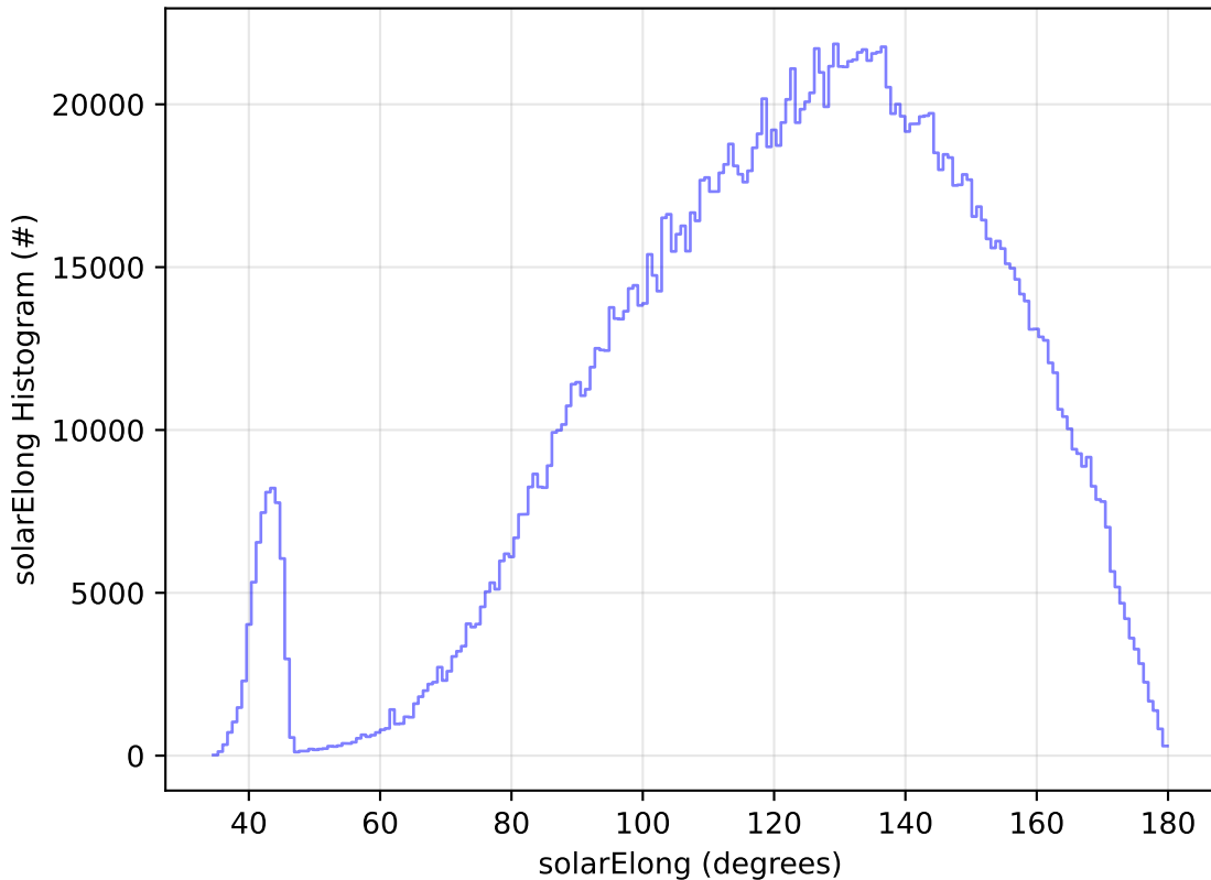
ddf_acor_sf20_lsf0_lsr0_v3.4_10yrs WFD all bands: solarElong Histogram
