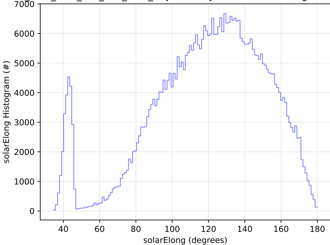
ddf_acor_sf20_lsf0_lsr0_v3.4_10yrs All sky z band: solarElong Histogram
