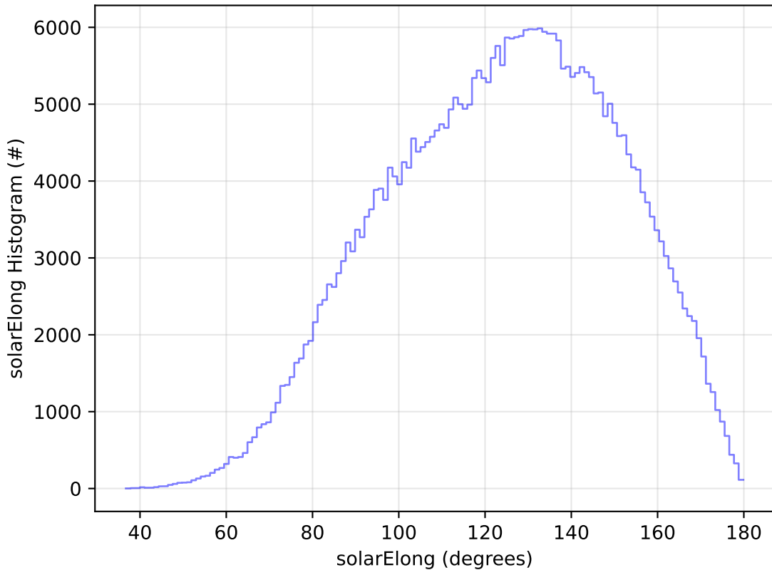
ddf_acor_sf20_lsf0_lsr0_v3.4_10yrs All sky y band: solarElong Histogram
