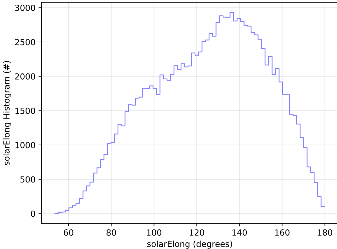
ddf_acor_sf20_lsf0_lsr0_v3.4_10yrs All sky u band: solarElong Histogram
