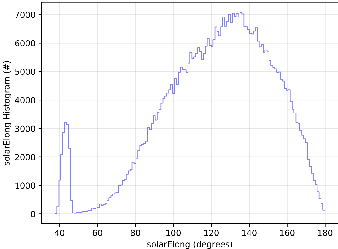
ddf_acor_sf20_lsf0_lsr0_v3.4_10yrs All sky r band: solarElong Histogram
