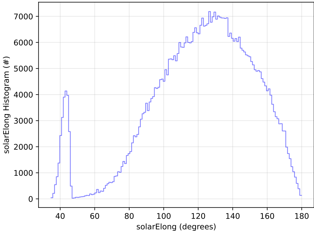
ddf_acor_sf20_lsf0_lsr0_v3.4_10yrs All sky i band: solarElong Histogram
