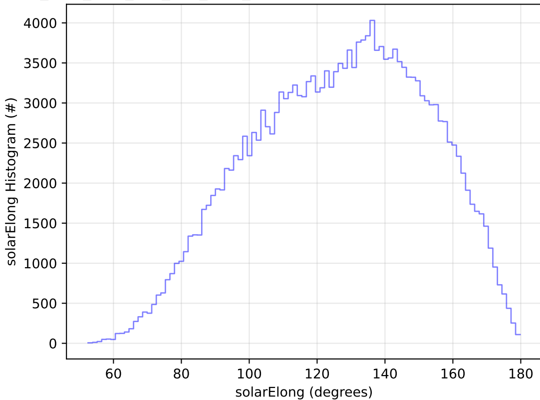
ddf_acor_sf20_lsf0_lsr0_v3.4_10yrs All sky g band: solarElong Histogram
