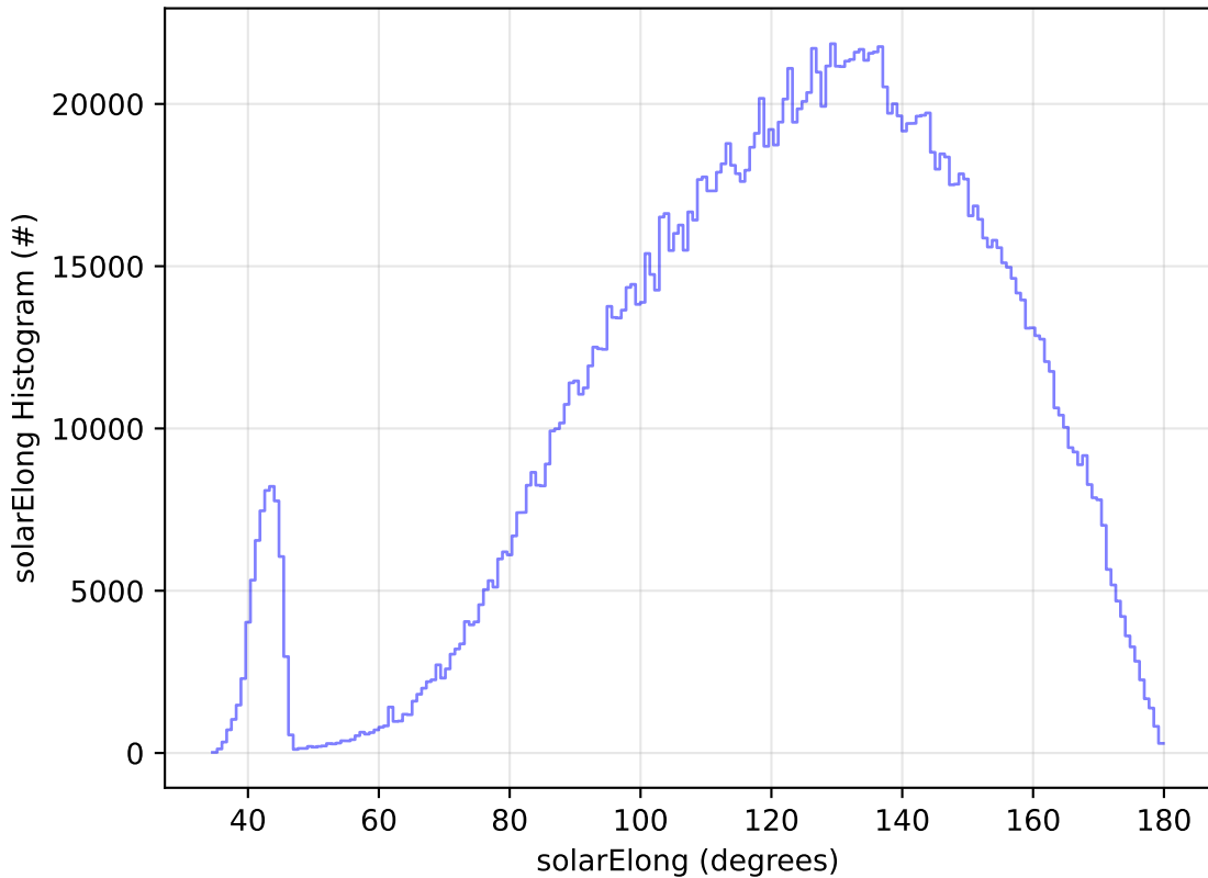
ddf_acor_sf20_lsf0_lsr0_v3.4_10yrs All sky all bands: solarElong Histogram
