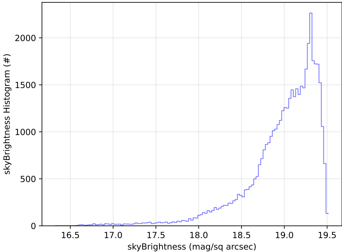
ddf_acor_sf20_lsf0_lsr0_v3.4_10yrs Yr 1 z band: skyBrightness Histogram
