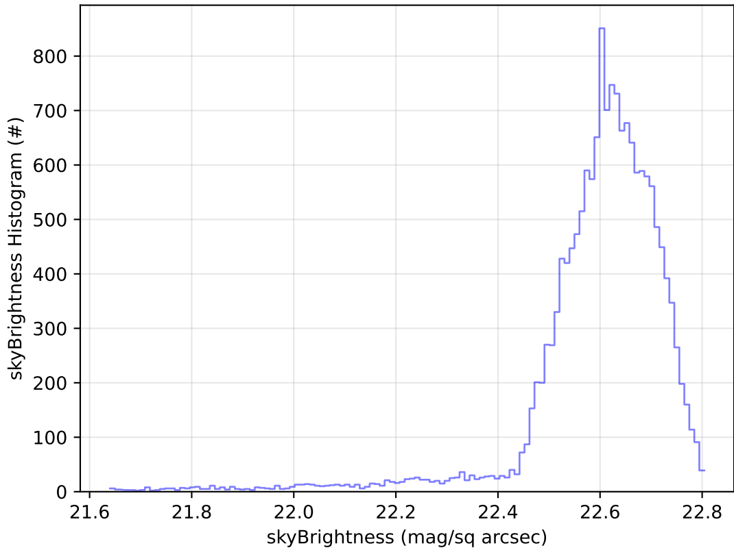
ddf_acor_sf20_lsf0_lsr0_v3.4_10yrs Yr 1 u band: skyBrightness Histogram
