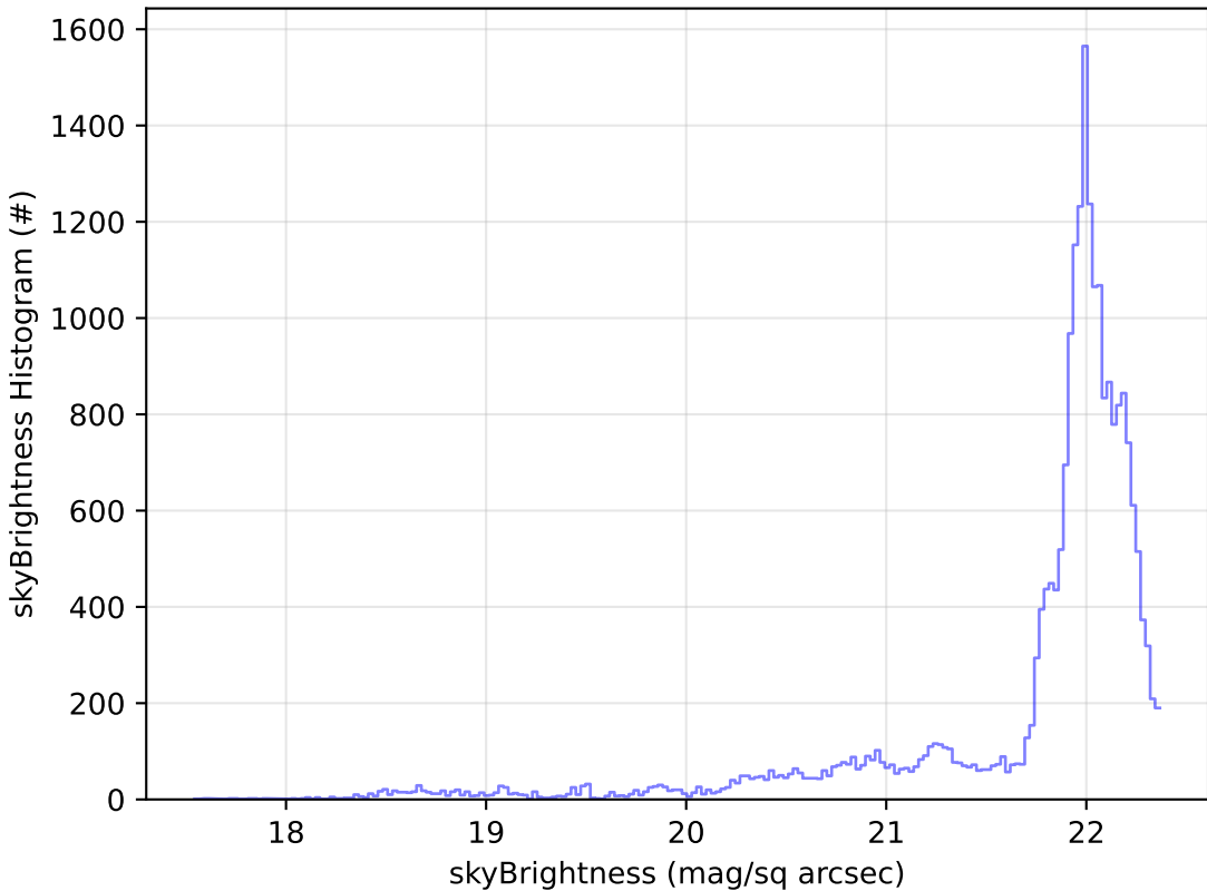
ddf_acor_sf20_lsf0_lsr0_v3.4_10yrs Yr 1 g band: skyBrightness Histogram
