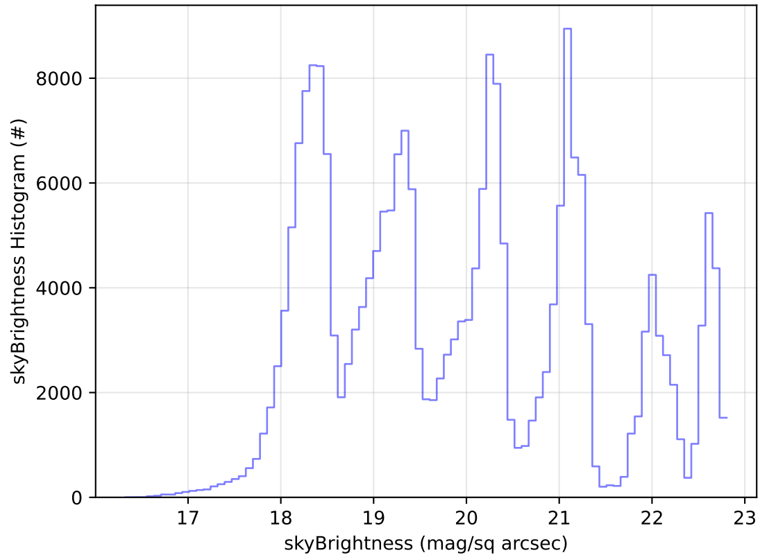
ddf_acor_sf20_lsf0_lsr0_v3.4_10yrs Yr 1 all bands: skyBrightness Histogram
