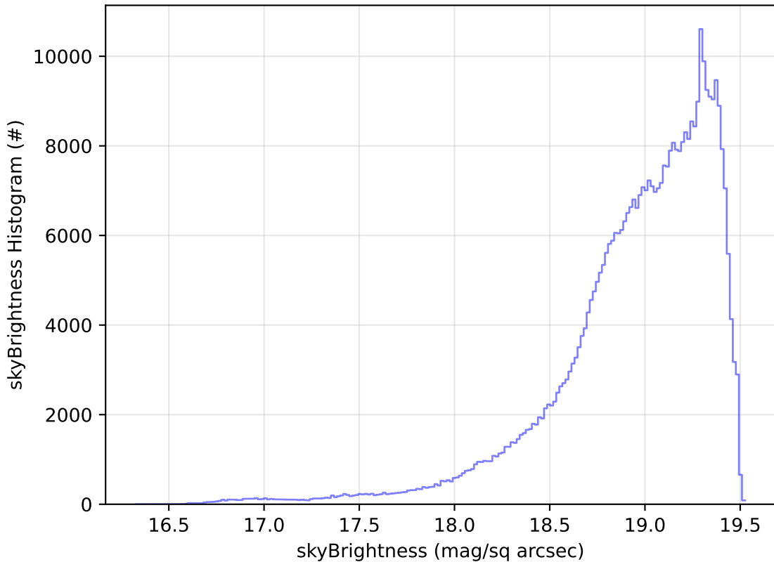
ddf_acor_sf20_lsf0_lsr0_v3.4_10yrs WFD z band: skyBrightness Histogram
