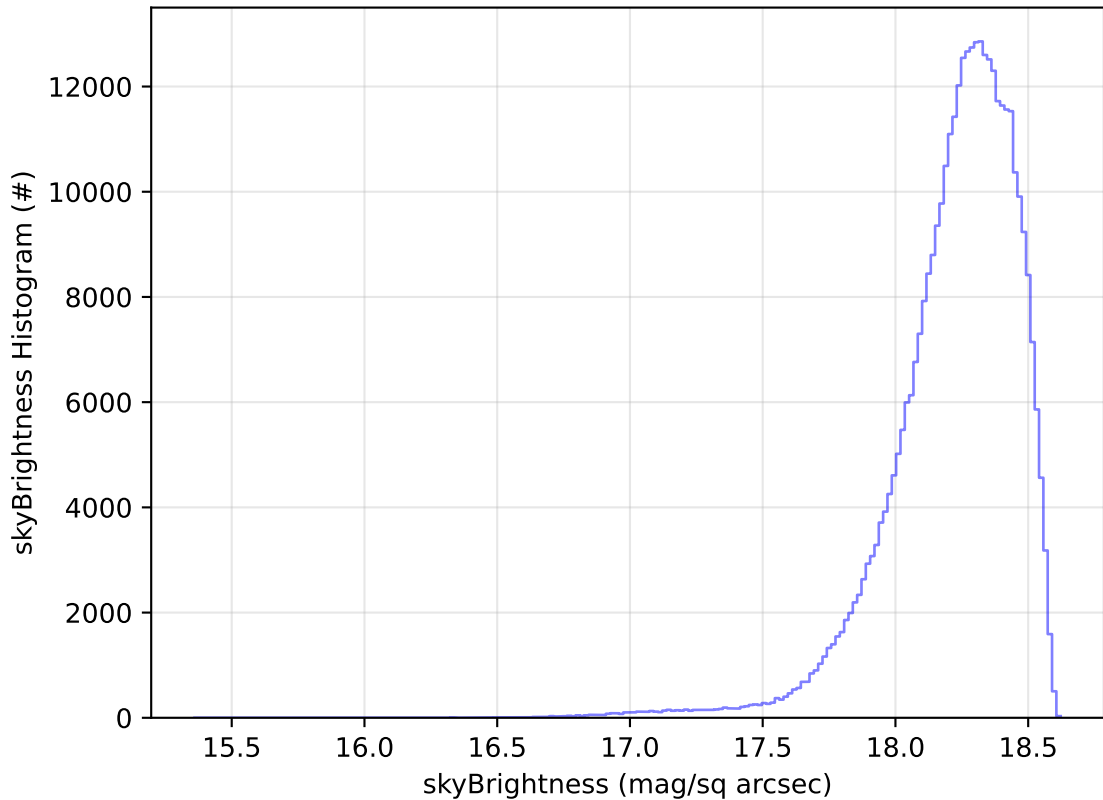
ddf_acor_sf20_lsf0_lsr0_v3.4_10yrs WFD y band: skyBrightness Histogram
