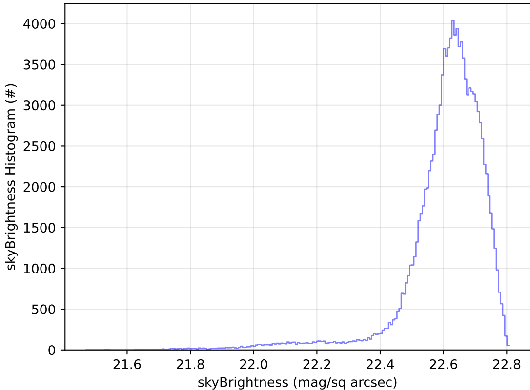
ddf_acor_sf20_lsf0_lsr0_v3.4_10yrs WFD u band: skyBrightness Histogram
