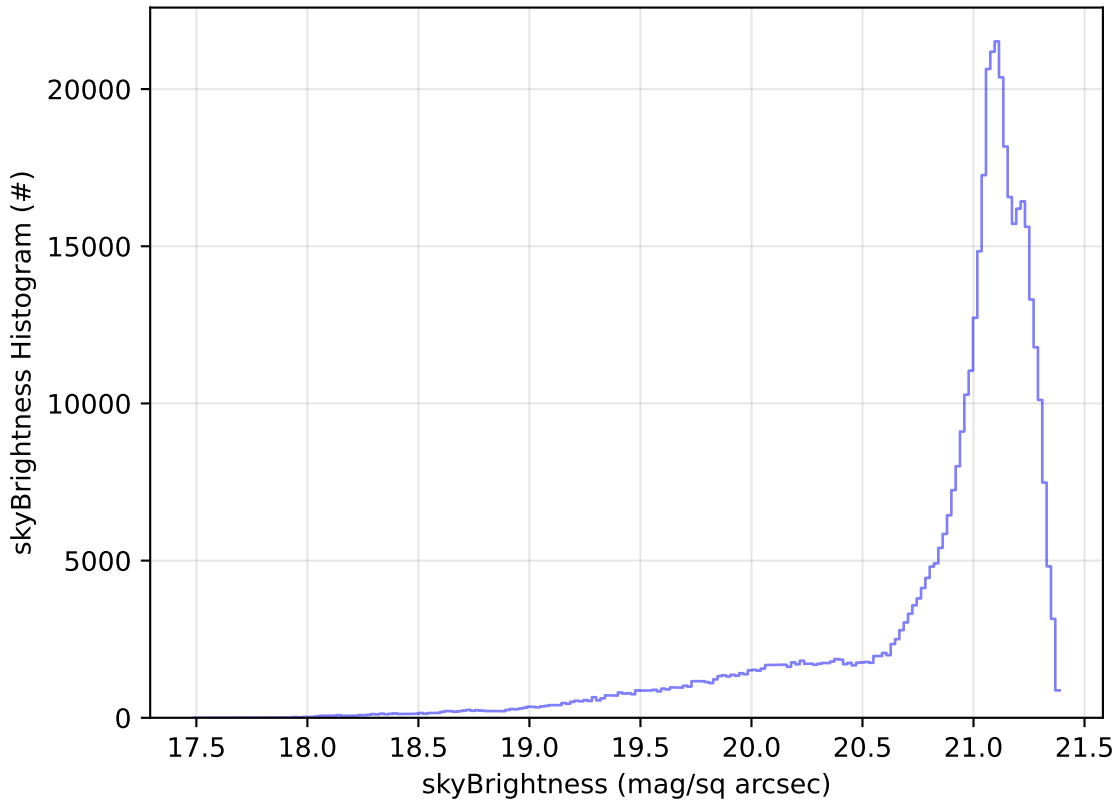
ddf_acor_sf20_lsf0_lsr0_v3.4_10yrs WFD r band: skyBrightness Histogram
