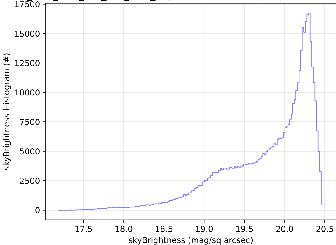
ddf_acor_sf20_lsf0_lsr0_v3.4_10yrs WFD i band: skyBrightness Histogram
