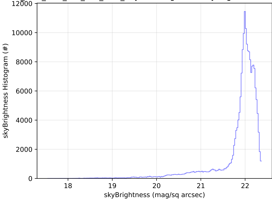
ddf_acor_sf20_lsf0_lsr0_v3.4_10yrs WFD g band: skyBrightness Histogram
