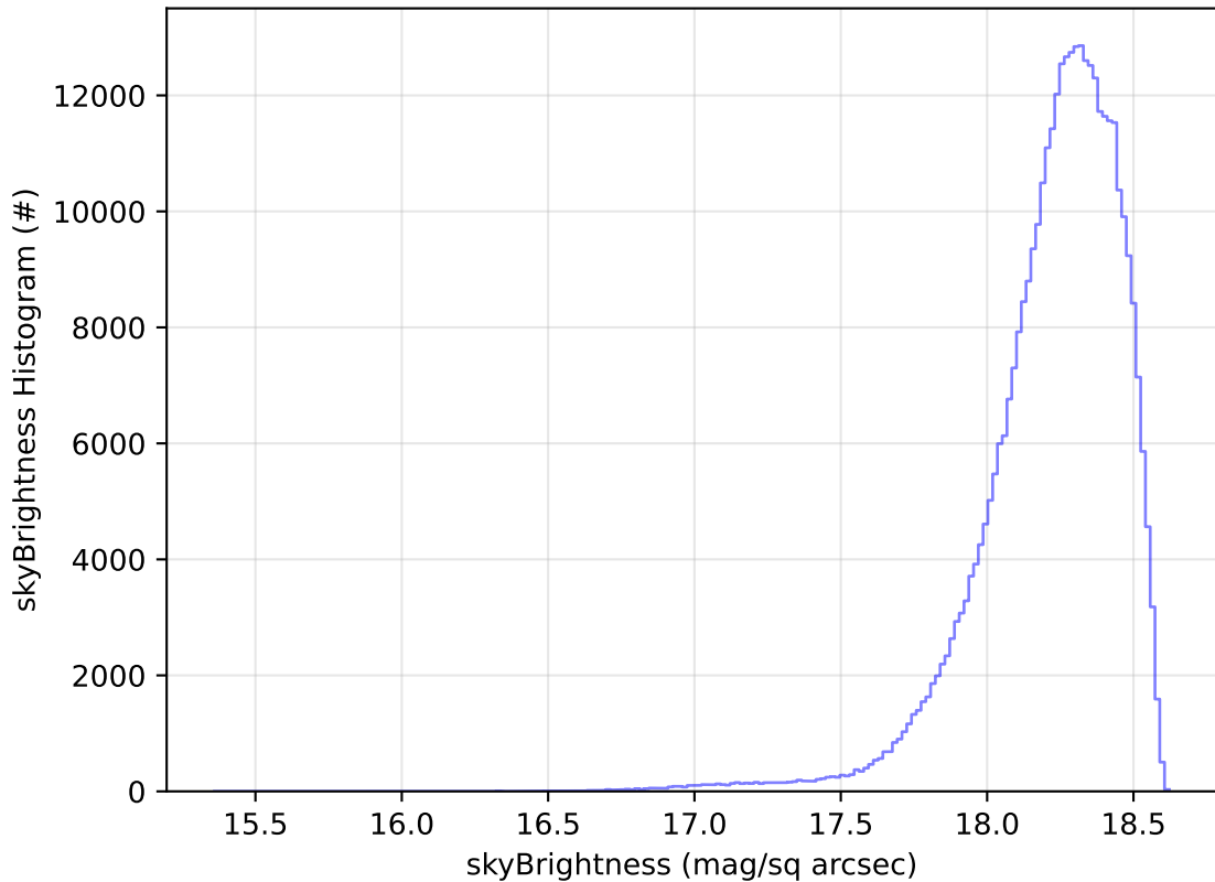
ddf_acor_sf20_lsf0_lsr0_v3.4_10yrs All sky y band: skyBrightness Histogram
