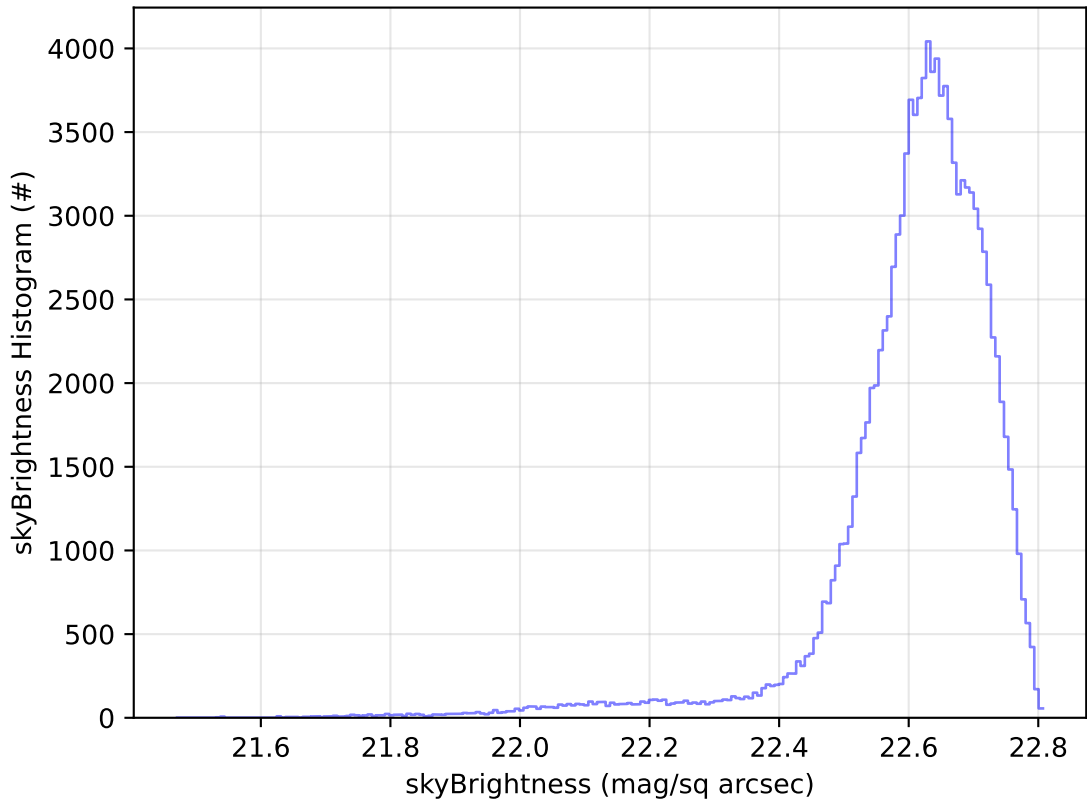
ddf_acor_sf20_lsf0_lsr0_v3.4_10yrs All sky u band: skyBrightness Histogram
