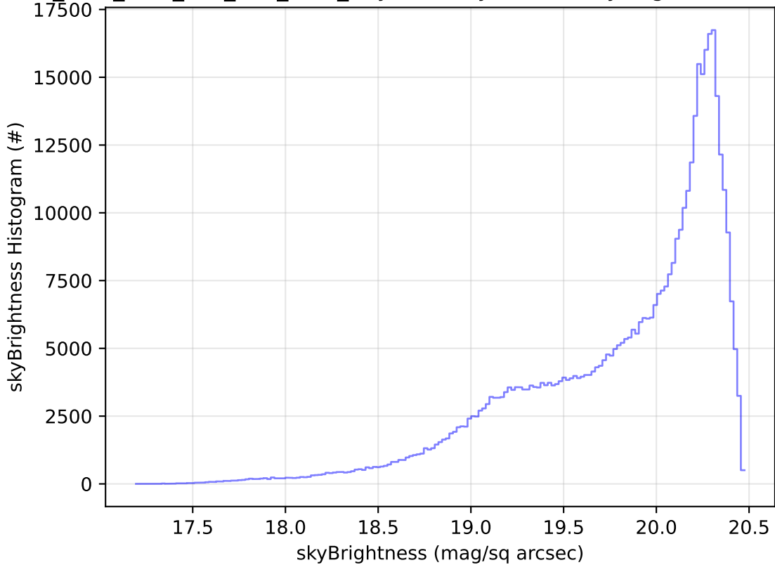
ddf_acor_sf20_lsf0_lsr0_v3.4_10yrs All sky i band: skyBrightness Histogram
