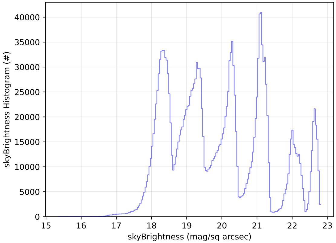
ddf_acor_sf20_lsf0_lsr0_v3.4_10yrs All sky all bands: skyBrightness Histogram
