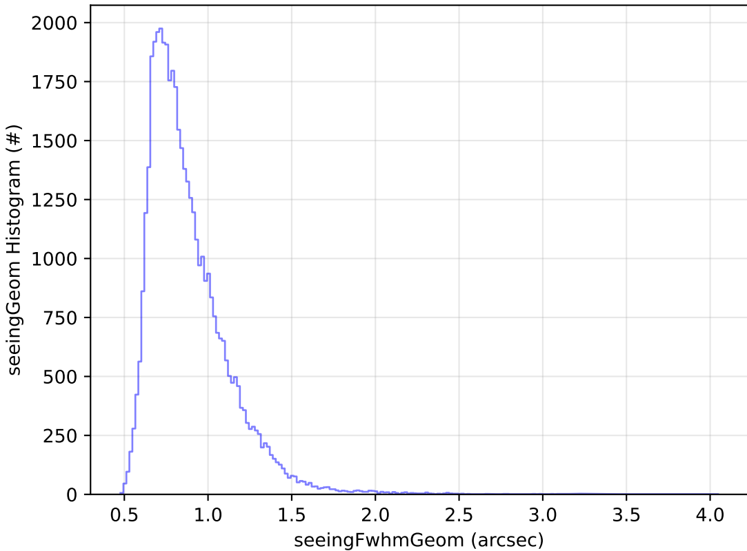
ddf_acor_sf20_lsf0_lsr0_v3.4_10yrs Yr 1 z band: seeingGeom Histogram
